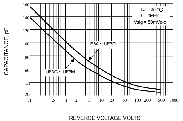
Fig. 6-TYPICAL JUNCTION CAPACITANCE
