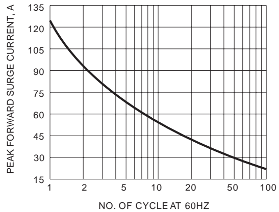
Fig.4- MAXIMUM ON-REPETITIVE SURGE CURRENT
