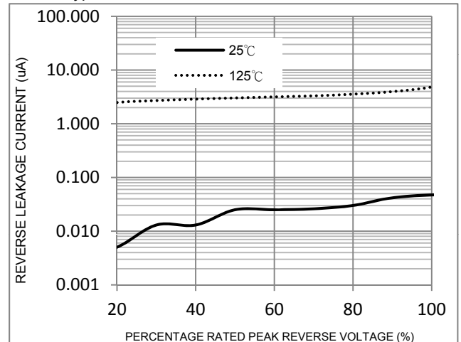
FIG. 4-Typical Reverse Characteristics
