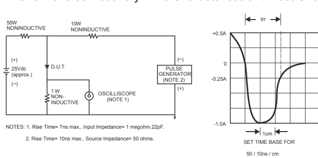
FIG. 6-Reverse Recovery Time Characteristic and Test Circuit
