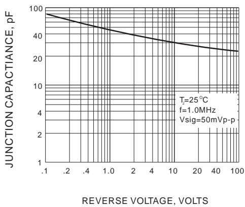
Fig.4-TYPICAL JUNCTION CAPACITANCE
