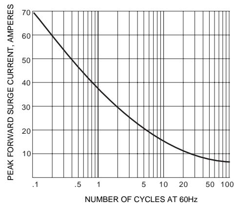
Fig.5-MAXIMUM NON-REPETITIVE PEAK FORWARD SURGE CURRENT
