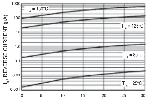
Figure 3. Leakage Current
