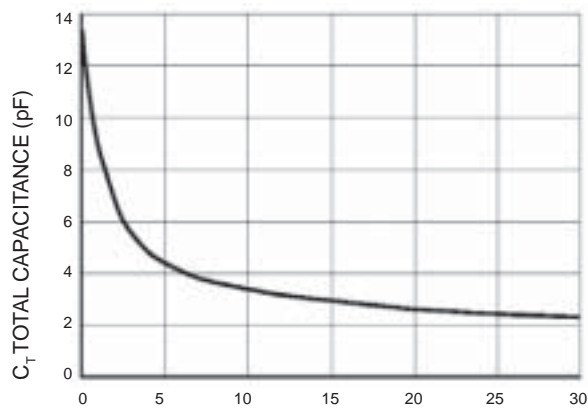
Figure 4. Total Capacitance
