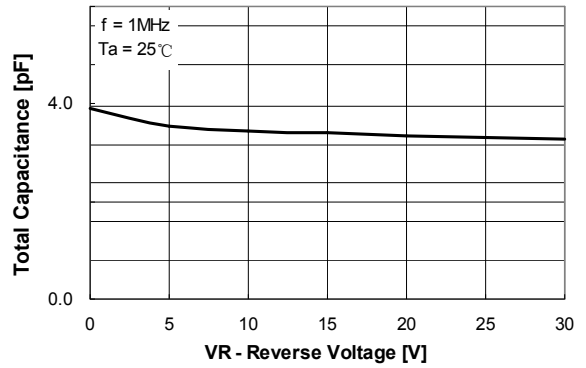
Figure 2. Total Capacitance
